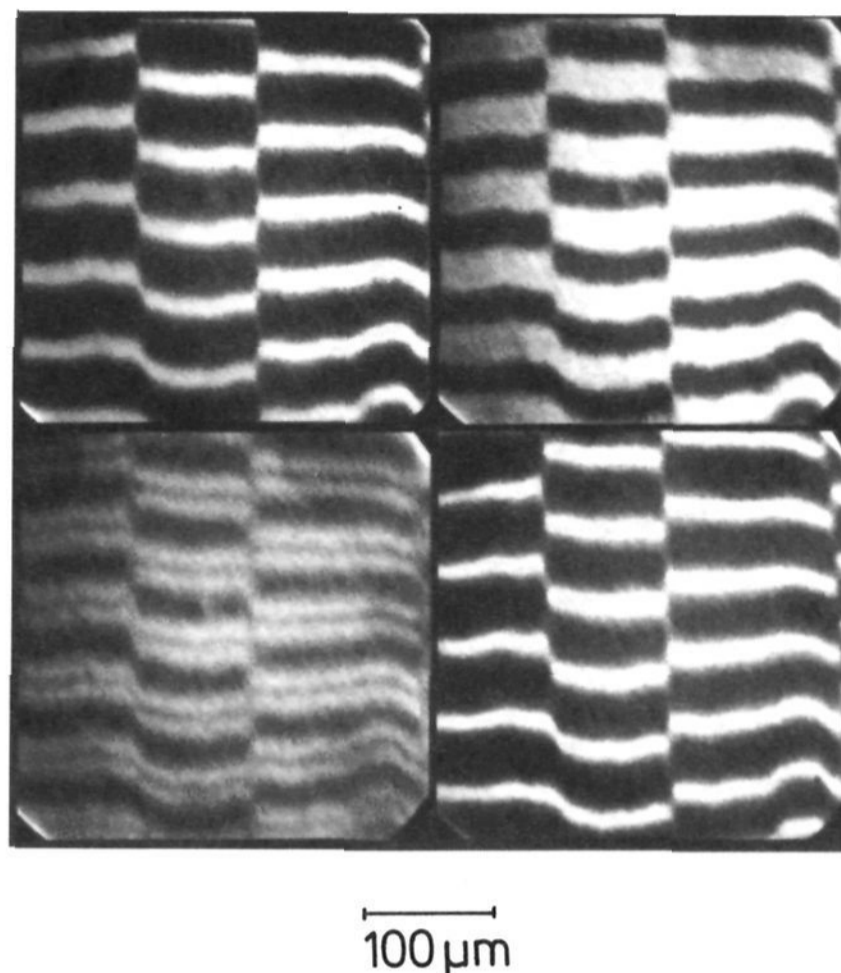
Figure 22. Standing wave patterns accompanying rapid kinetic oscillations in CO oxidation on a Pt(110) surface. The PEEM images which represent an area of 0.3 \times 0.5 mm 2 were recorded at intervals of 0.5 s. Experimental conditions: T = 550 K, p_{\text{O}_2} = 4.1 \times 10^{-4} mbar, p_{\text{CO}} = 1.75 \times 10^{-4} mbar. (Reprinted from ref 82. Copyright 1990 American Institute of Physics.)
