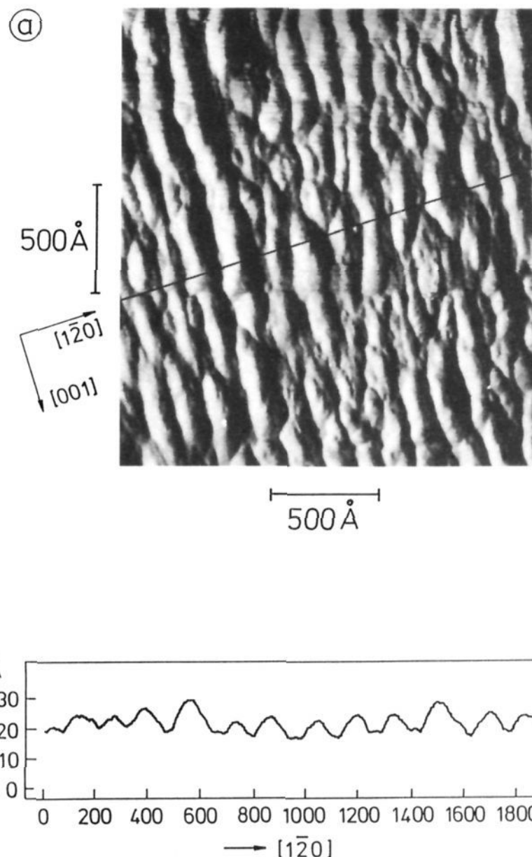
Figure 11. STM image (a) of a Pt(210) surface which had been faceted during catalytic CO oxidation. The surface had been exposed for 1 h at T = 480 K to CO and O_2 at 10^{-4} mbar. A profile cut in the (120) direction is shown in b. (Reprinted from ref 186. Copyright 1992 J. C. Baltzer AG.)
