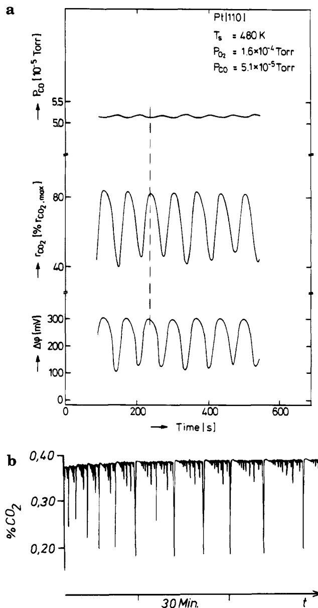
Figure 2. Some examples of different wave-forms of rate oscillations in catalytic CO oxidation: (a) kinetic oscillations in catalytic CO oxidation on Pt(110) measured via the variation of the CO 2 partial pressure p_{\text{CO}_2} and the work function variation \Delta\phi and (b) self-similar pattern observed in catalytic CO oxidation at atmospheric pressure and T = 453 K with a Pd/zeolite catalyst. (a: Reprinted from ref 78. Copyright 1990 American Institute of Physics. b: Reprinted from ref 28. Copyright 1986 Chemical Society of London.)
